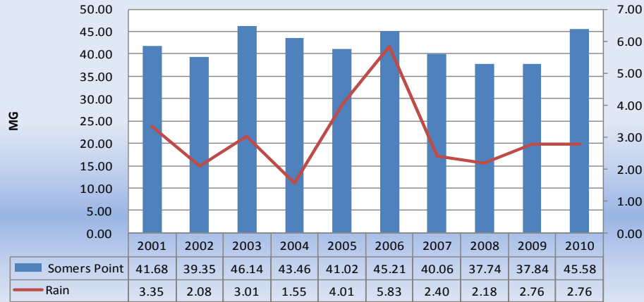
Somers Point March Flow
