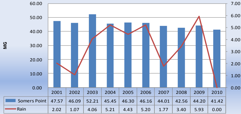
Somers Point September Flow
